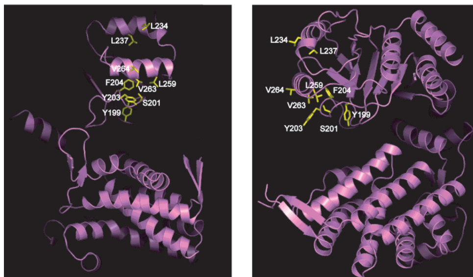
Figure 3. Apical peptide binding surface of a GroEL subunit. Ribbons model shows hydrophobic side chains exposed to solvent, mapping onto three secondary structures, from top to bottom, Helix H, Helix I, and underlying segment, viewed from central cavity, left, and from the side, right. Mutational change of any one of these residues (seven within a ring) abolishes polypeptide binding by GroEL.
