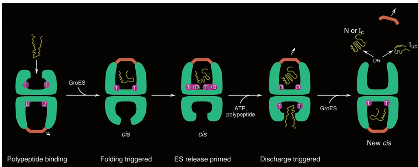
Figure 6. GroEL–GroES reaction cycle. Asymmetric GroEL–GroES–nucleotide complexes are likely the predominant states in the cell. A GroEL–GroES–ADP asymmetric complex binds a non-native substrate polypeptide in a collapsed, largely unstructured state via hydrophobic interactions with its apical domains (panel a), an action that may result in further unfolding of the substrate. Binding of ATP (either before polypeptide or thereafter; the relative rates of arrival have not been measured) followed by GroES to the same ring as polypeptide (panel b) results in large-scale conformational changes of the GroEL apical domains, which move the hydrophobic sites away from the cavity surface and permit GroES to cap the GroEL ring, forming a cis folding-active complex. Concomitant with the ATP/GroES-driven apical movements, polypeptide is ejected into the central cavity (<1 s), where it begins to fold in this sequestered chamber whose walls are now hydrophilic in character. This wall character favors burial of hydrophobic side chains of the substrate protein and exposure of its hydrophilic ones, characteristic of the native state. Folding continues in this longest-lived state of the cycle until ATP hydrolysis in the cis ring (panel c), occurring with a half-time of about 8–10 s, weakens the cis complex and permits ATP (and non-native polypeptide) binding to the trans ring (panel d). This rapidly allosterically discharges the ligands from the cis ring (panel e) (<1 s), regardless of the folding state of the substrate polypeptide. The released polypeptide may have folded to its native state (N) or one committed to it ( I_c ), or it may have failed to reach the native state ( I_{uc} ), in which case it can be bound to GroEL again for another attempt at folding. GroES binding to the same ring as ATP and polypeptide forms a new cis complex on the previous trans ring to begin the cycle again. Thus, GroEL alternates its rings between binding-active and folding-active states, using one round of seven ATPs to simultaneously discharge one folding-active complex while forming another. Note that an asymmetric ATP complex has no significant affinity of its trans ring for any of the ligands, whereas once cis ATP hydrolysis occurs, it can accept non-native polypeptide and ATP, and, in an ATP-bound state, can now bind GroES.
