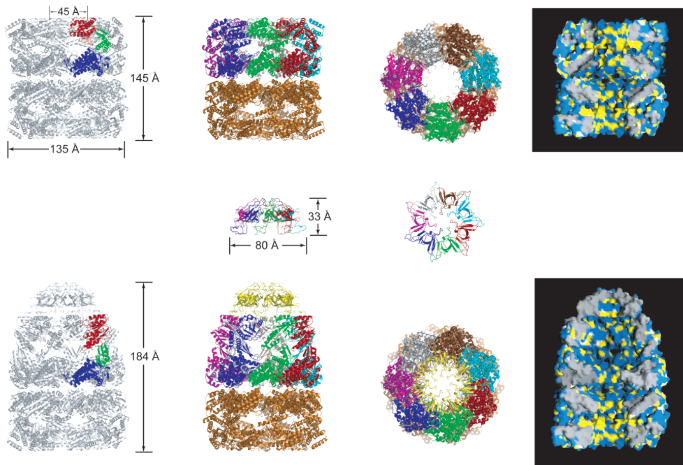
Figure 2. Architecture of the bacterial chaperonin system, GroEL and GroES. Crystallographic models of GroEL, GroES, and GroEL–GroES complexes are shown in the top, middle, and bottom rows, respectively (pdb1oel and 1aon). Left column, a single subunit of GroEL is colored in GroEL and GroEL–GroES: apical domain, red; equatorial domain, blue; intermediate domain, green. Second column, assemblies with GroEL and GroES subunits colored individually in selected rings. Third column, subunits colored individually in end views looking down the central cavity, which measures \sim 45 Å in diameter. Note, however, that this cavity is obstructed at the equatorial level in both rings by flexible C-terminal tails of each GroEL subunit that are not resolvable crystallographically (see text). Fourth column, space-filling model colored to illustrate hydrophobicity (yellow) and hydrophilicity (blue).
