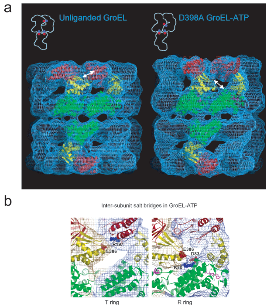
Figure 4. Action of ATP binding in a GroEL ring (in the absence of GroES), comparing unliganded GroEL, left images, and an ATP-bound hydrolysis defective mutant, D398A, right images, by cryoEM image reconstruction. 58 The top images show that ATP produces downward rotational movement of the intermediate domain accompanied by modest elevation and twisting movement of the apical domains of the ATP bound ring, shown as the top ring. The downward movements of the intermediate domain break a salt bridge between E386 and R197 of the neighboring subunit, lower left panel, and E386 forms a new contact with K80 at the top aspect of the neighboring equatorial domain. The broken 386–197 bridge allows the apical domains to move freely, enabling their elevation and twist. Note that the direction of twist is \sim 15^\circ counterclockwise, opposite to the direction taken upon GroES binding, which totals, from this position, 120^\circ clockwise. Reprinted with permission from ref 58. Copyright 2001 Elsevier.
